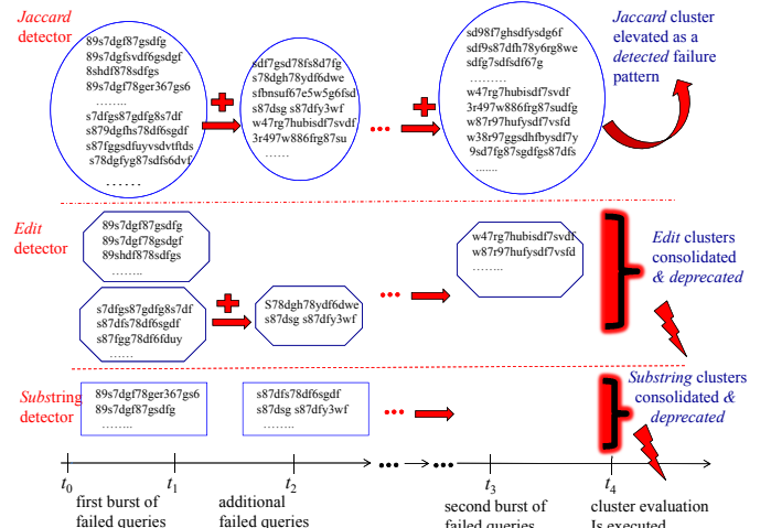
Fig. 5. Framework illustration using an example.
